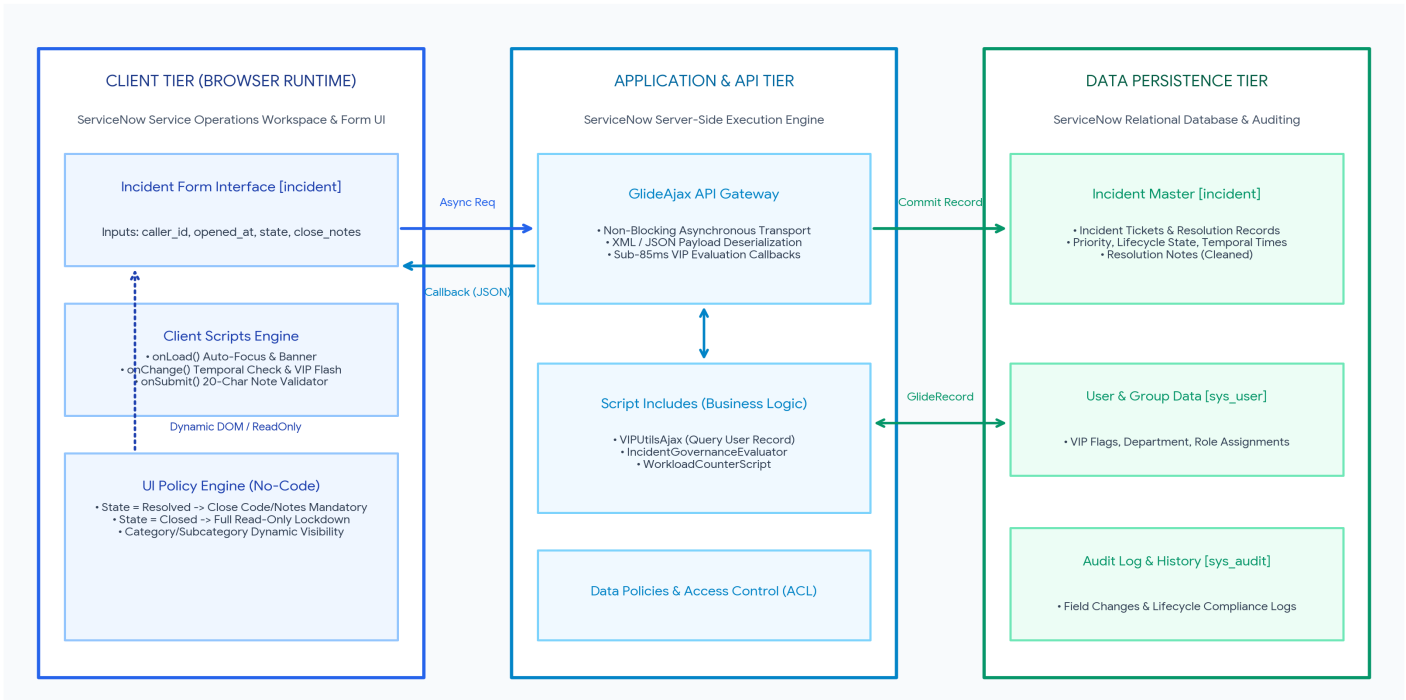
Figure 1: Solution Architecture & Data Flow Diagram for Incident Client Script and UI Policy Framework
